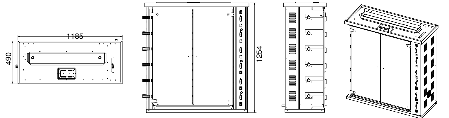
HDSROG-6
